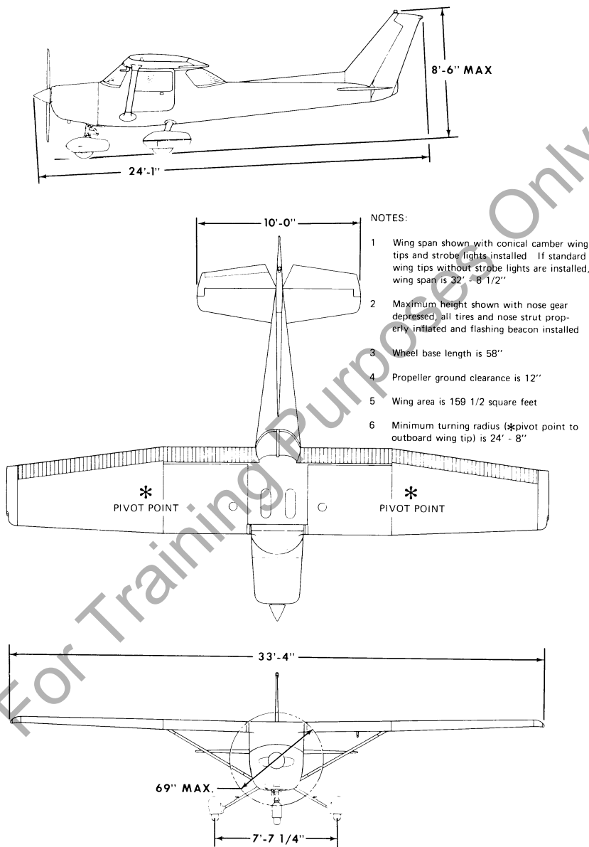
Figure 1-1. Three View
