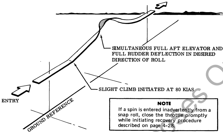
Figure 4-9. Snap Roll
