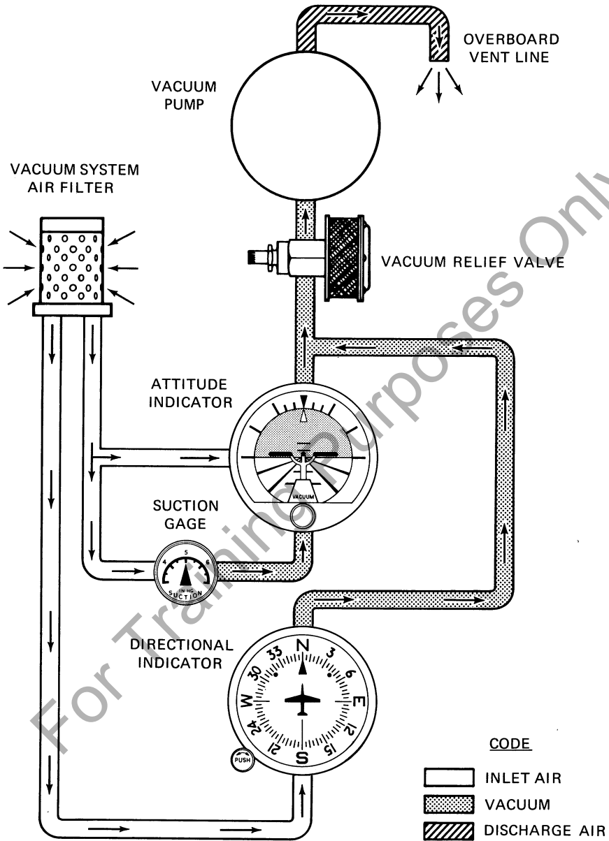
Figure 7-9. Vacuum System
