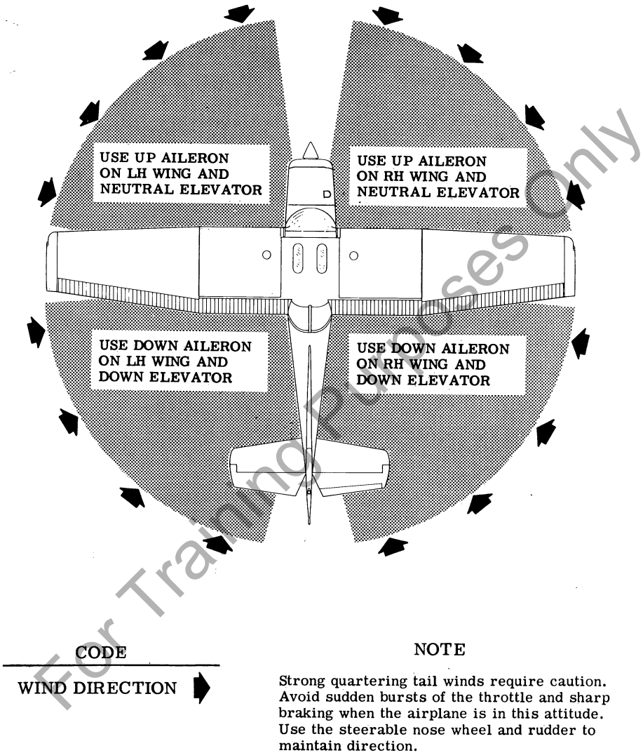
Figure 4-2. Taxiing Diagram
