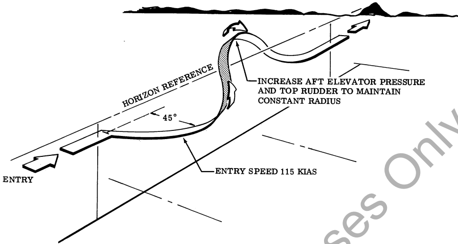
Figure 4-7. Barrel Roll
