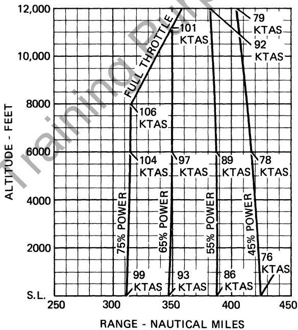
Figure 5-8. Range Profile (Sheet 1 of 2)
