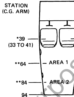
Figure 6-3. Loading Arrangements
