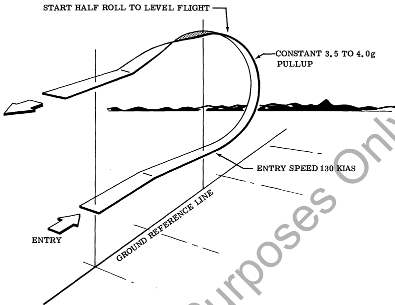
Figure 4-11. Immelmann
