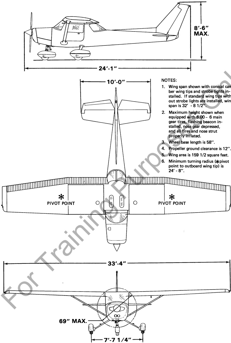
Figure 1-1. Three View
