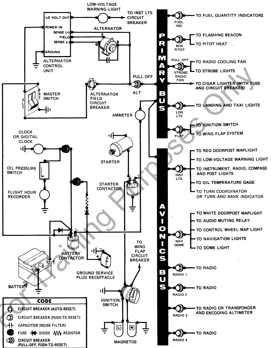
Figure 7-7. Electrical System
